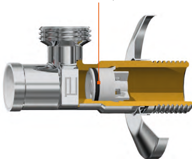
Sistema auto-stop Auto shut-off system
